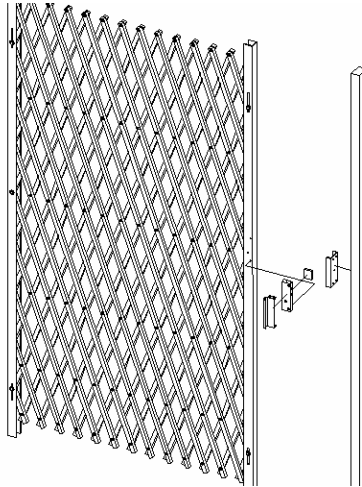
Figure 1-Overview of Installation
