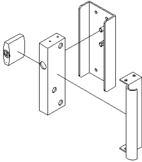
Figure 3-Lock Assembling Step 2
